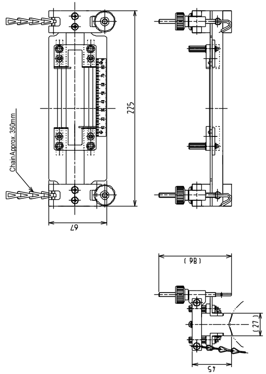
Fixture for small transducer
