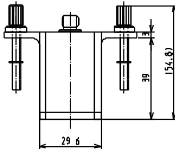
Medium transducer
