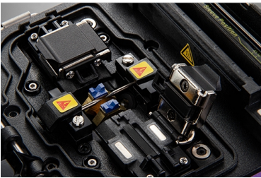
Easy removable holder for SOC Real-time ARC calibration
